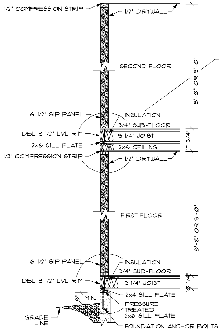
TYPICAL TWO STORY FLOOR TO FLOOR SECTION
